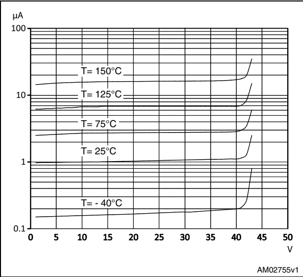
Figure 3. Reverse current
